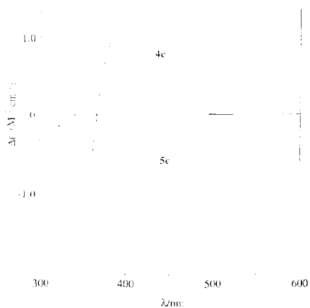
Fig. 1. CD spectra of 4c and 5c .
